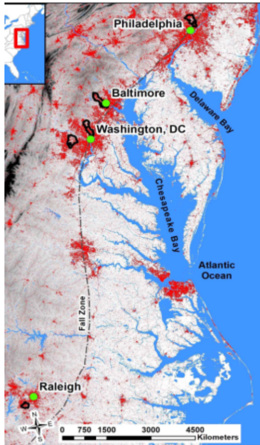
Network of Urban Critical Zone field sites located along the Fall Zone.
